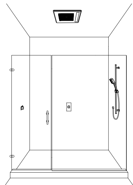
Configuration example for an optimal installation of the independent diverter (access the on/off control from outside the shower)
